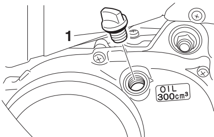
1. O-Ring
